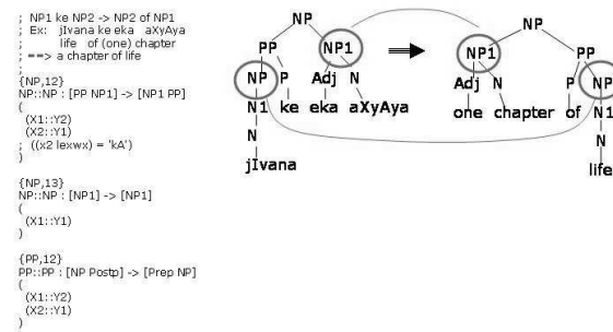
Figure 4. Recursive NP and PP Transfer Rules for Hindi to English Translation
