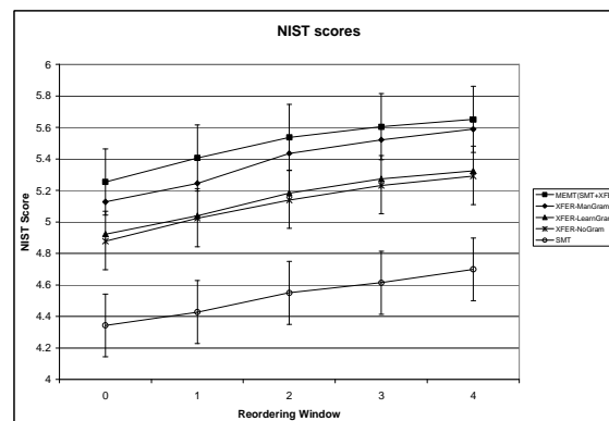
Figure 5. Results by NIST Score with Various Reordering Windows.
