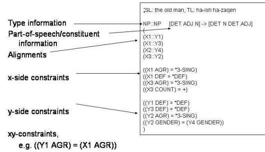
Figure 3. An Example Transfer Rule along with its Components
