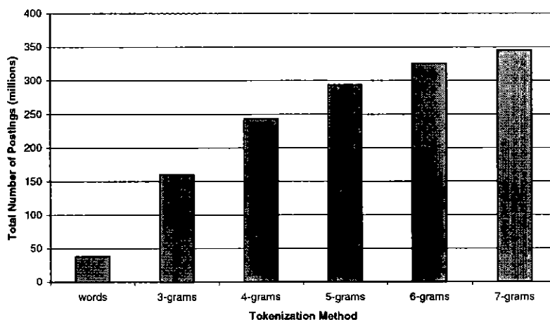
Figure 5. Size of inverted file for various tokenization methods.
