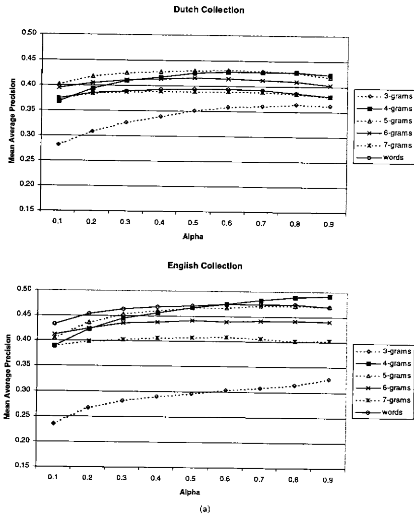
Figure 1. Comparative efficacy of n -gram indexing for eight languages.
