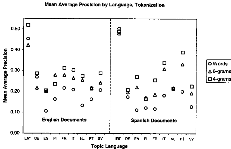
Figure 2. Using partial cognate matches for CLIR.
