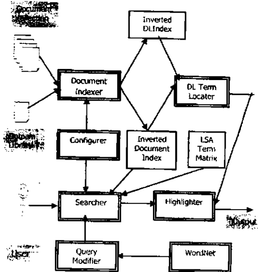
Figure 1. Architecture of Content-based Indexing and Semantic Search Engine
