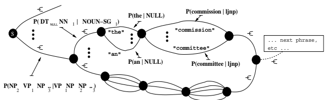
Figure 2: An illustration of the translation model structure for an Arabic test sentence. (a) The arcs immediately exiting the start state correspond to different sentence-level reordering possibilities. These arcs have, as attached weights, the probability of the particular sentence-level reordering designated. (b) Other arcs in the machine correspond to phrase-level reorderings, as shown in the figure. For each of the Arabic phrases in the test sentence, there will be a distribution over possible English reorderings / POS-tag sequence generations, and arcs in the machine corresponding to different reordering/generation choices, with associated probabilities. (c) Finally, word translation is also represented by arcs in the machine. These are not epsilon arcs, but rather arcs that emit the particular English word translation in question, and which have the appropriate word-to-word translation probability attached to the arc.
